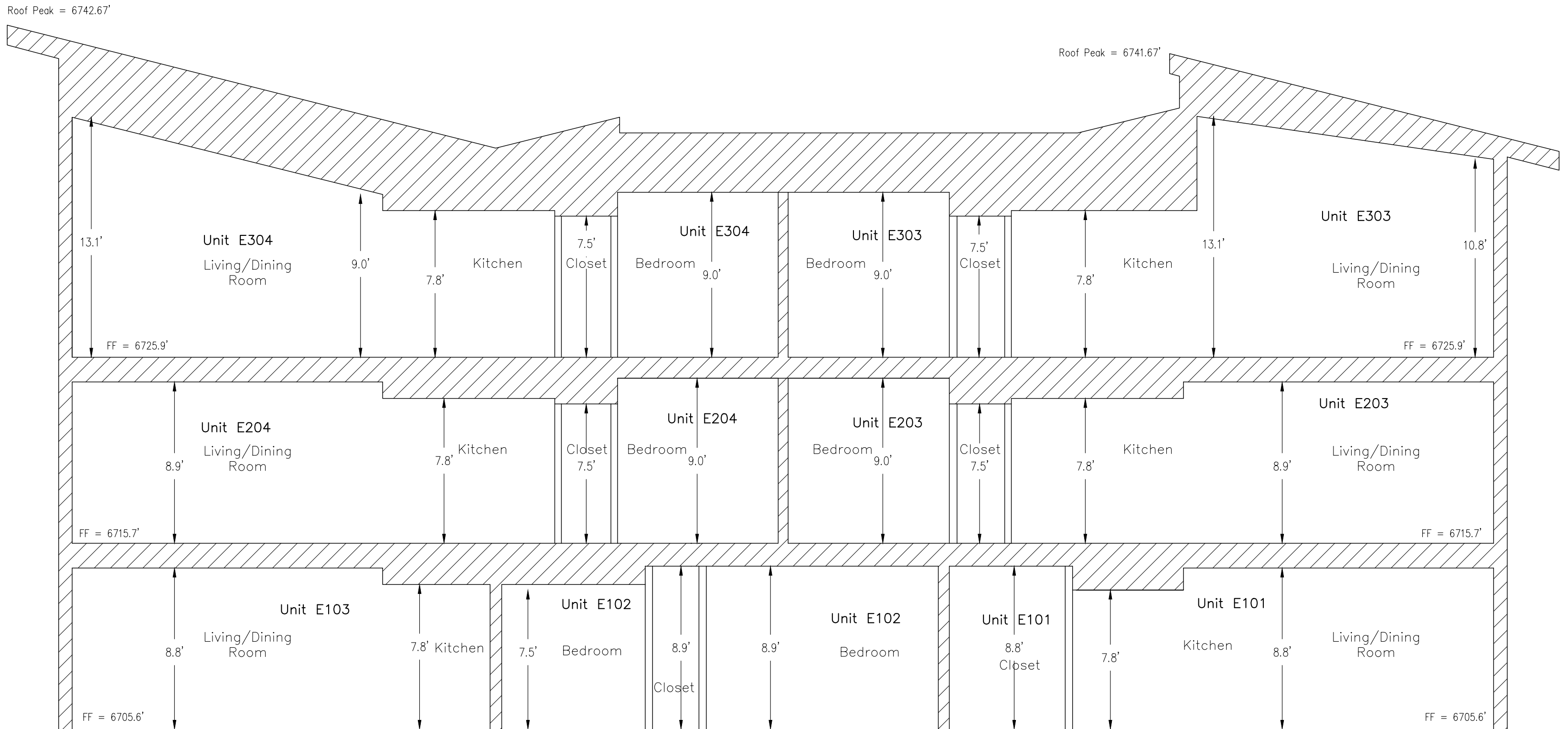
Building C Cross Section 2
