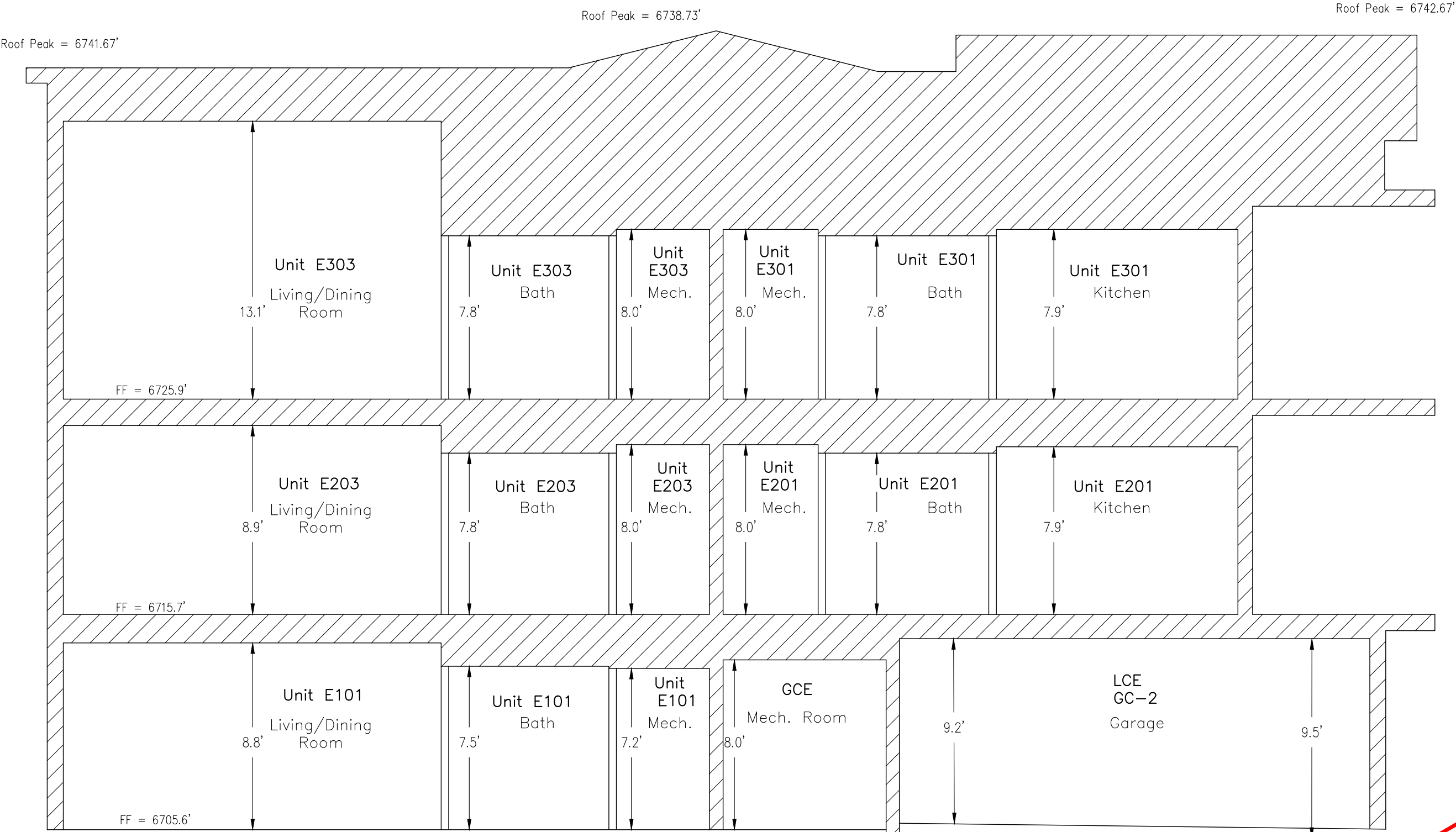
Building C Cross Section 4
