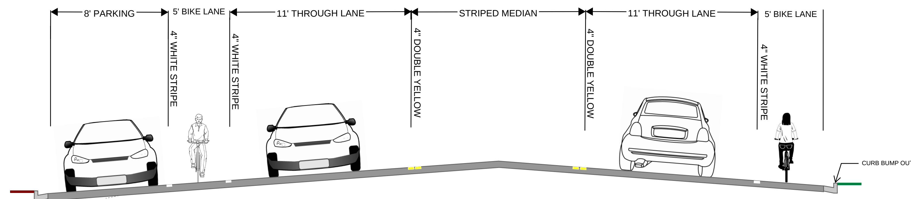
SYLVAN LAKE ROAD TYPICAL SECTION NOT TO SCALE
