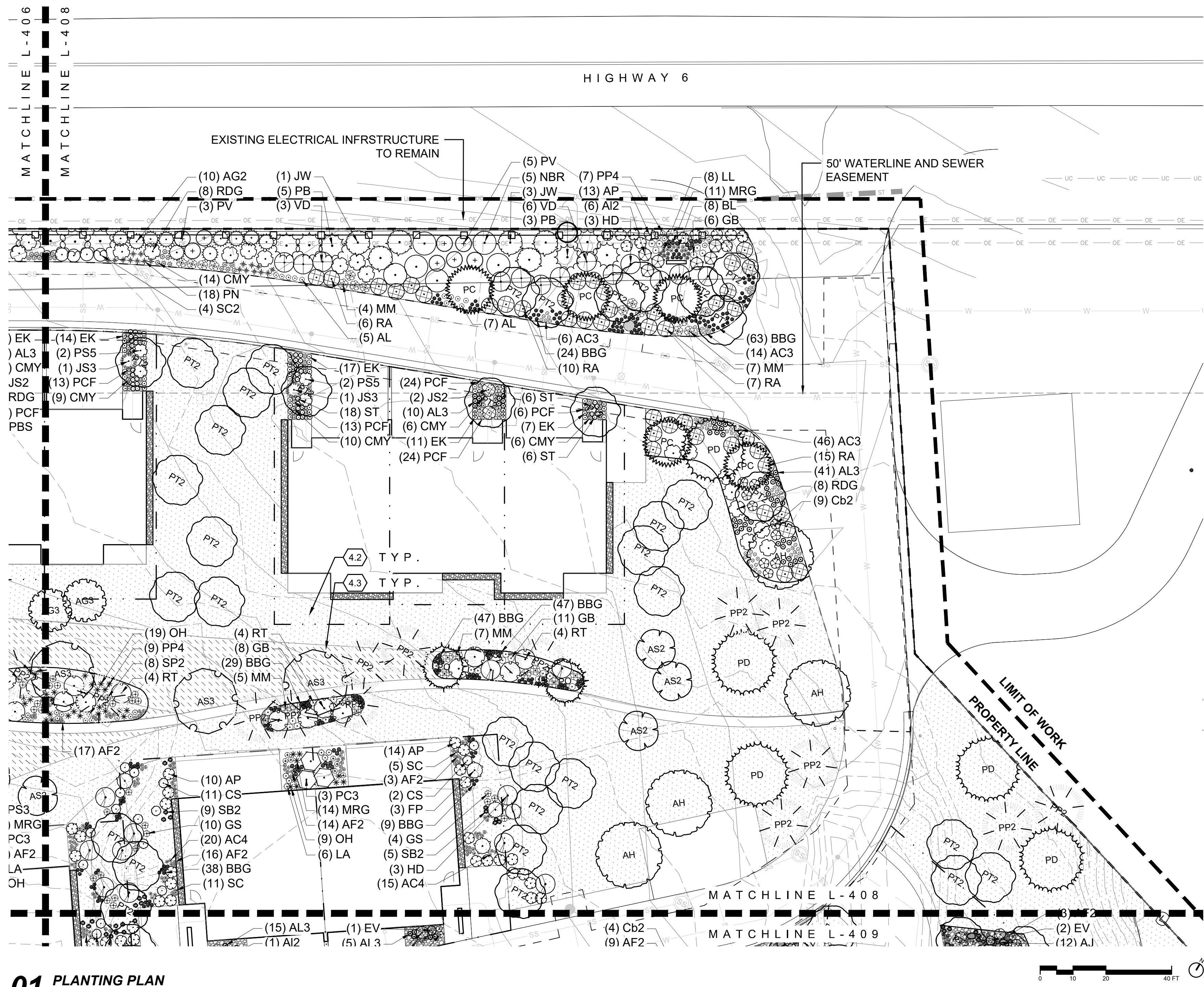
01 PLANTING PLAN 1"=20'
