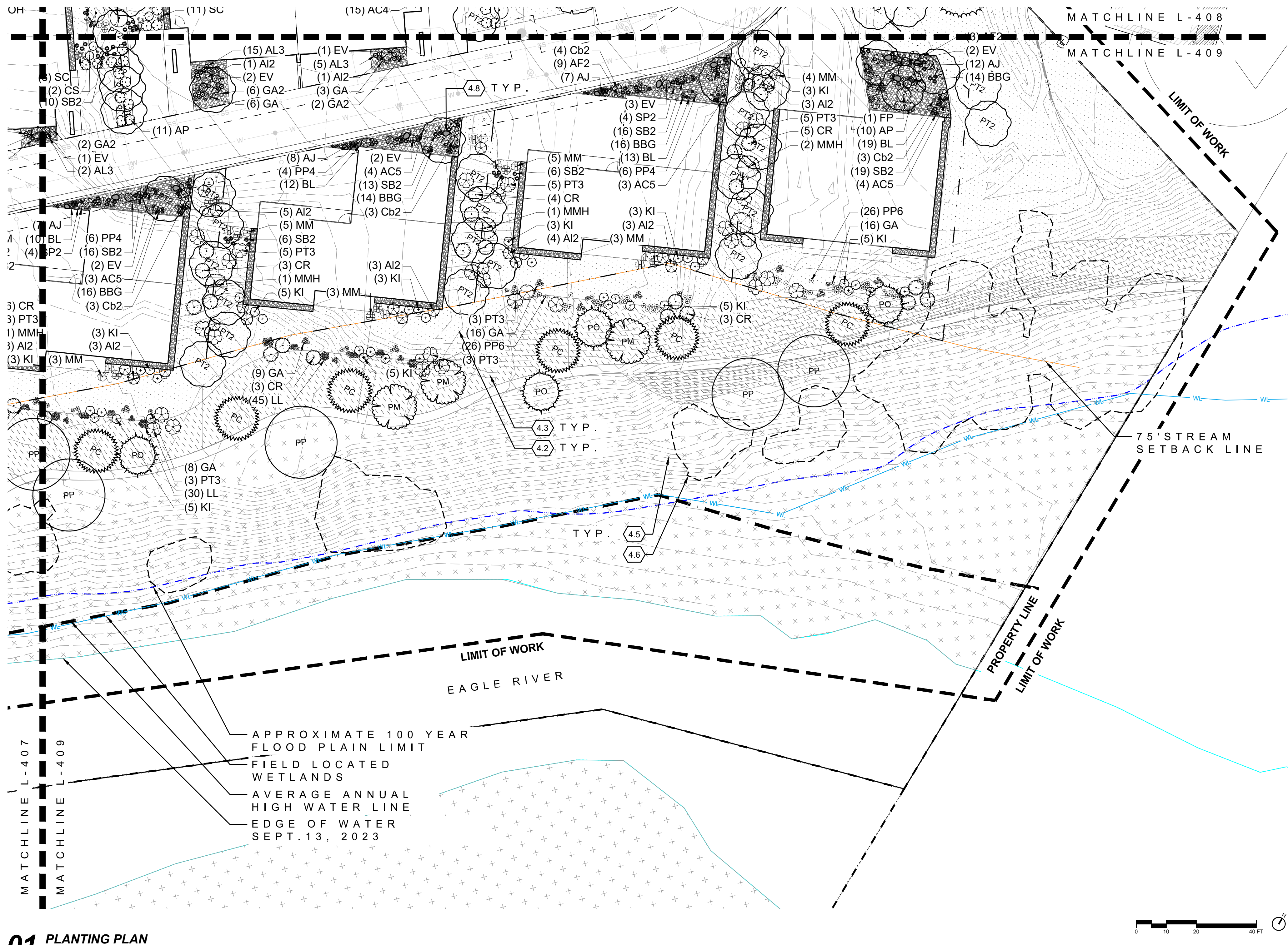
01 PLANTING PLAN 1"=20'
