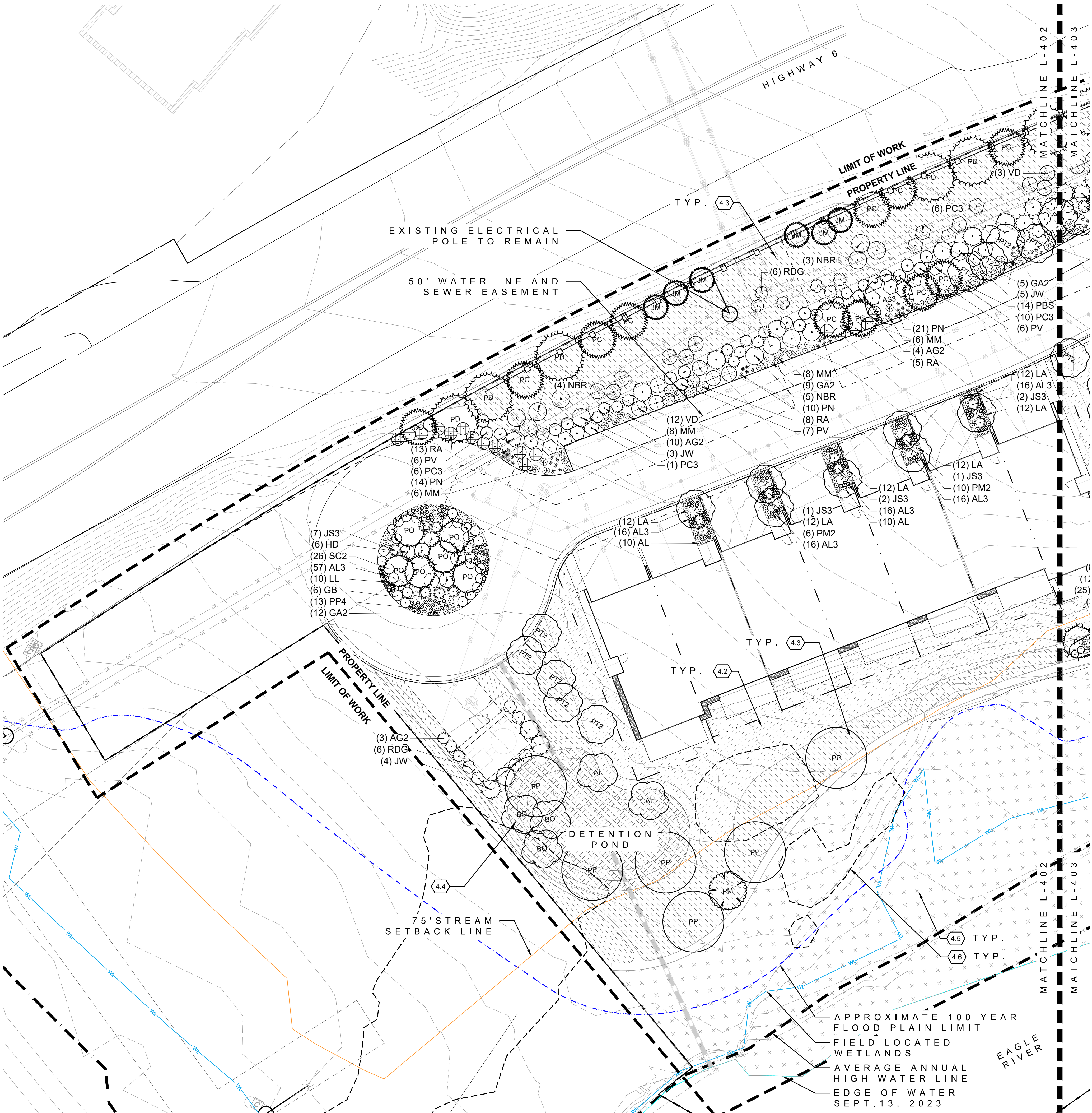
01 PLANTING 1"=20'
