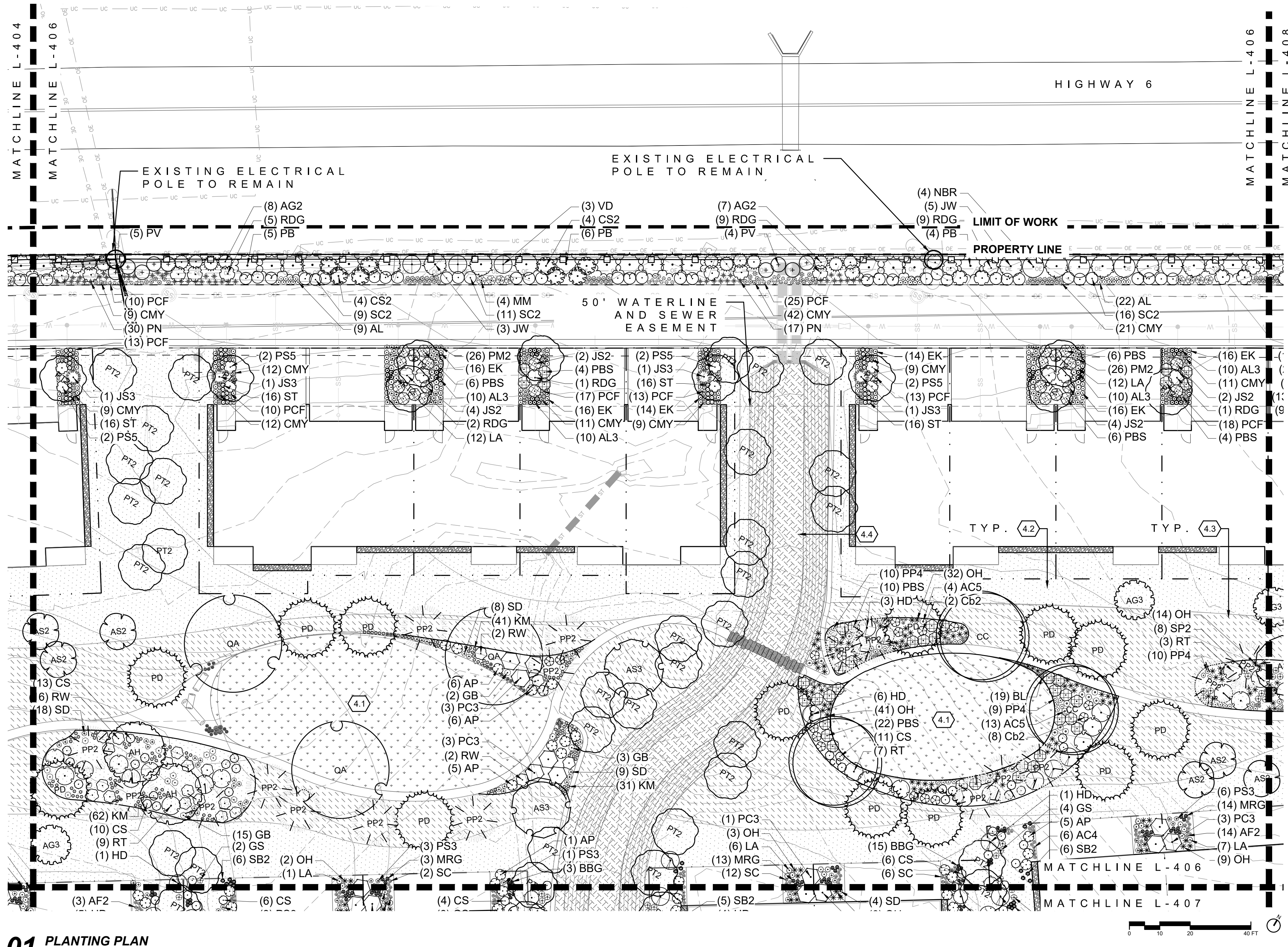
01 PLANTING PLAN 1"=20'
