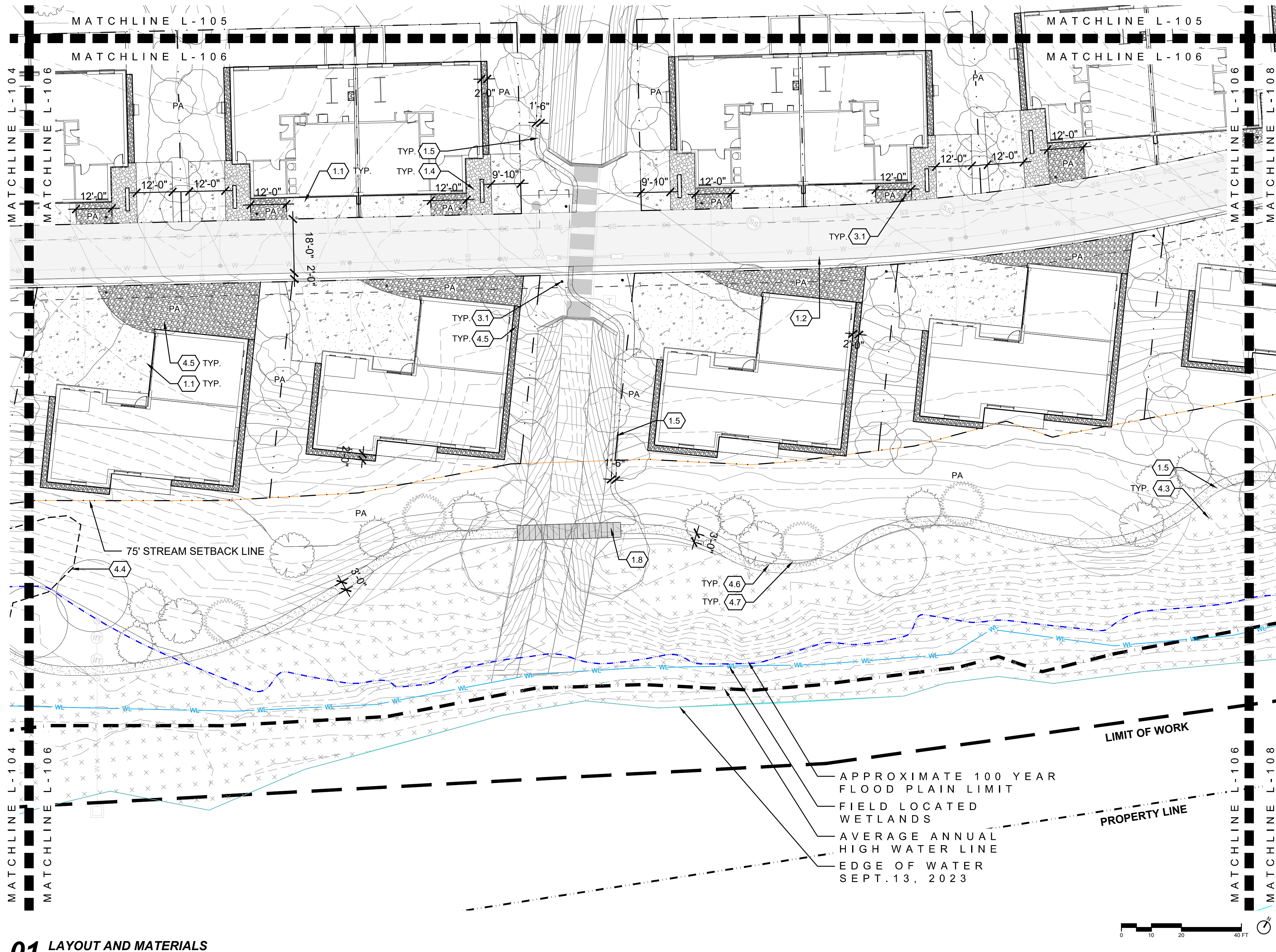
01 LAYOUT AND MATERIALS 1"=20'
